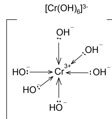
Hexahydroxochromium(III) ion
