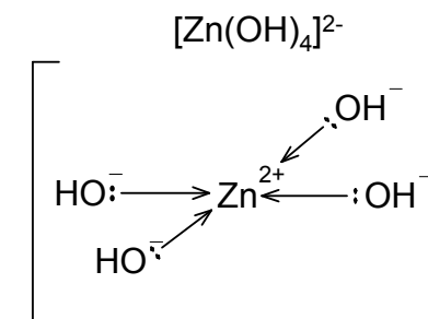
Tetrahydroxozincate(II) ion
