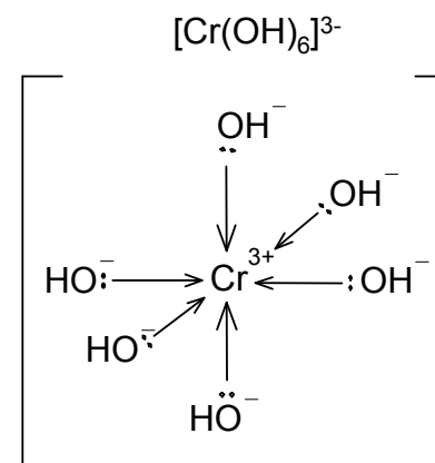
Hexahydroxochromium(III) ion
