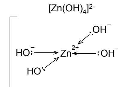
Tetrahydroxozincate(II) ion
