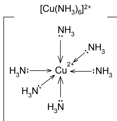
Hexaamminecopper(II) ion
