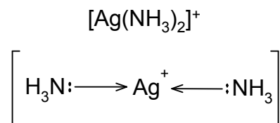
Diamminesilver(I) ion
