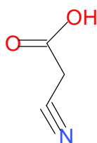
2-cyanoacetic acid
