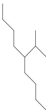
5-isopropylnonane
