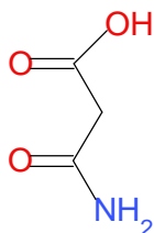
3-amino-3-oxo-propanoic acid
