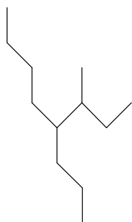
3-methyl-4-propyl-octane
