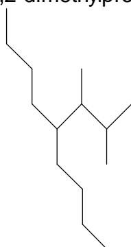
5-(1,2-dimethylpropyl)nonane
