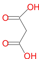
malonic acid
