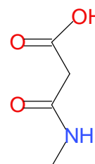
3-methylamino-3-oxo-propanoic acid
