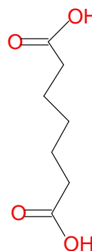
heptanedioic acid
