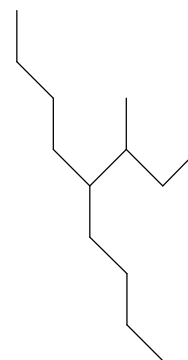
5-sec-butylnonane
